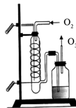
21-rasm. Ozonator.
