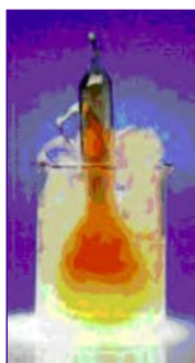
42-rasm. \text{NO}_2 ning gaz holati va muzli muhitdagi holati.
