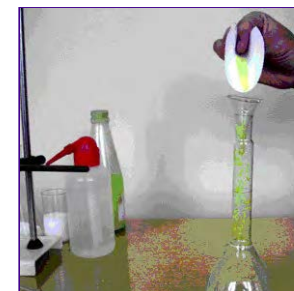
37-rasm. Modda eritmasini tayyorlash.
