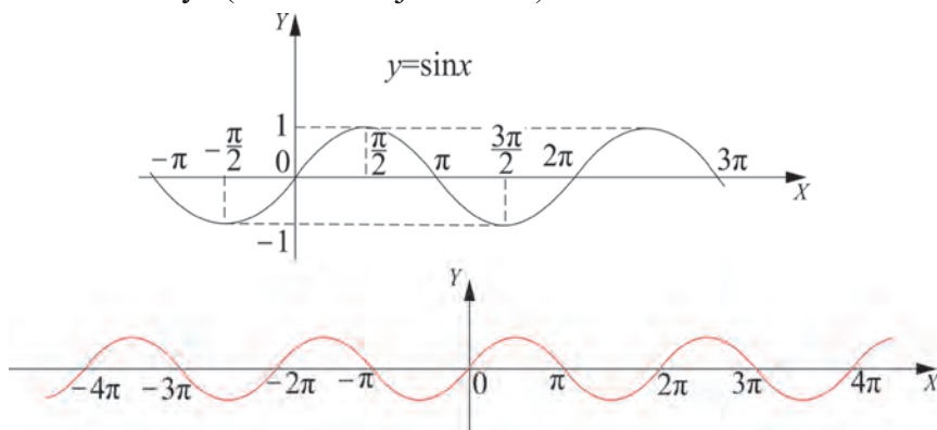
14-nji surat. y = \sin x , x \in \mathbb{R} .
