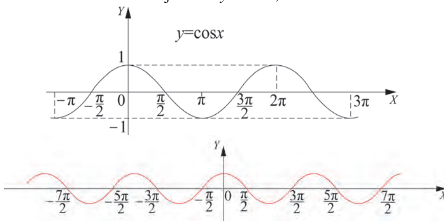
15-nji surat. y = \cos x , x \in \mathbb{R} .
