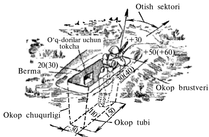
51-rasm. Avtomatdan turib otish uchun okop.
