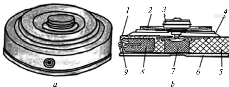
74-rasm. Tankka qarshi TM-57 mina MVZ-57 portlagich bilan birga ko'rinishi:
